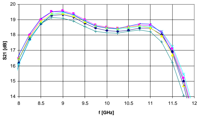
Small signal Gain ( V_d=8V , V_{g1}=-5V , P_s=-20dBm )
