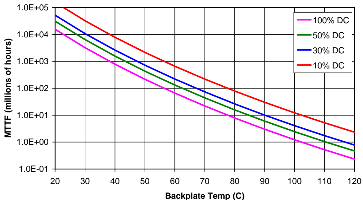
XP1014 MTTF vs. Backplate Temperature and Pulsed Duty Cycle
