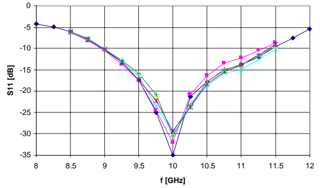
Input return loss ( V_d=8V , V_{g1}=-5V , P_s=17dBm )
