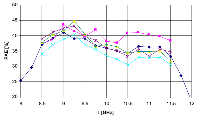
Power Added Efficiency ( V_d=8V , V_{g1}=-5V , P_s=17dBm )
